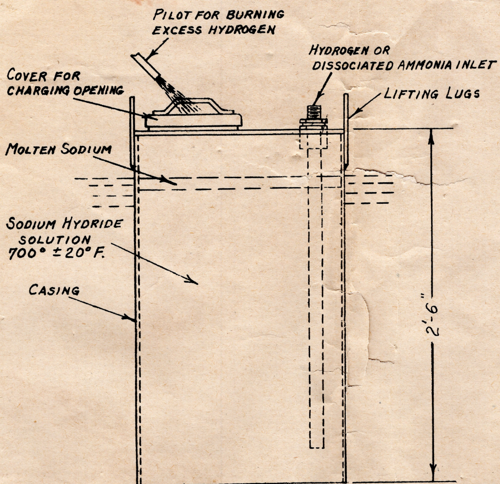
SODIUM HYDRIDE GENERATOR
