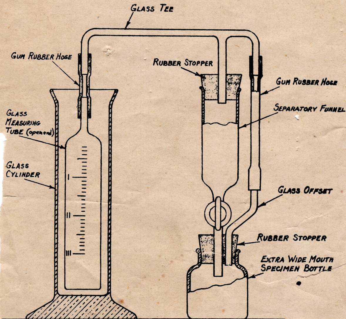
APPARATUS FOR TESTING CONCENTRATION OF SODIUM HYDRIDE SOLUTION
