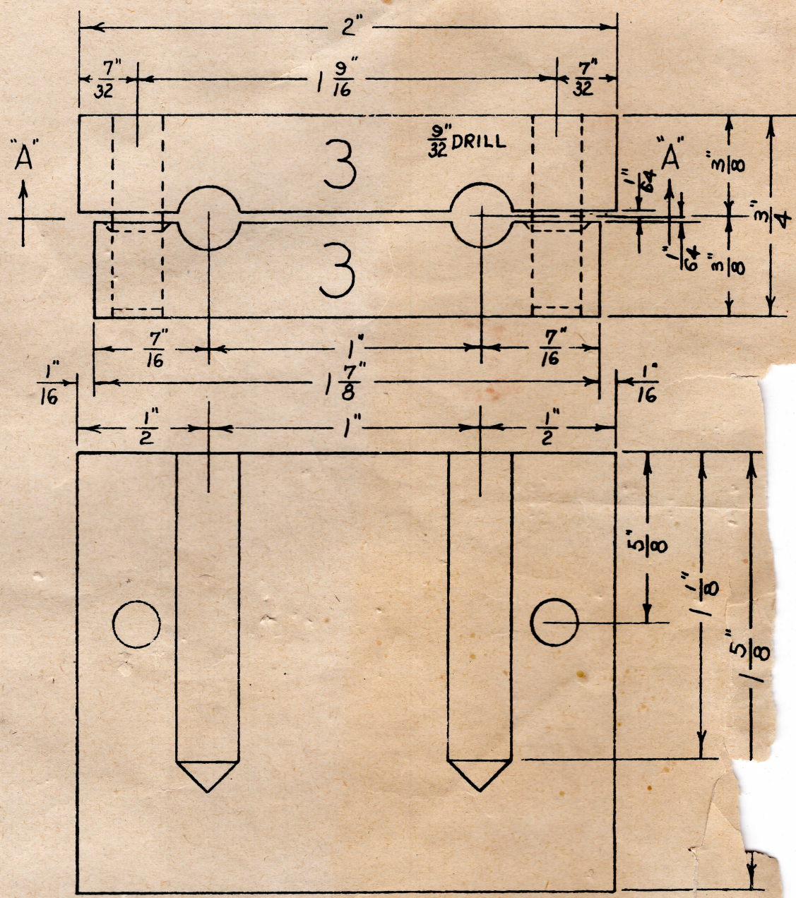
MOLD FOR SAMPLING SODIUM HYDRIDE SOLUTION
